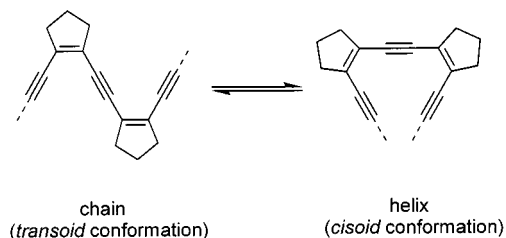
Figure 4. The backbone can adopt a transoid or a cisoid conformation by rotation about the triple bond
