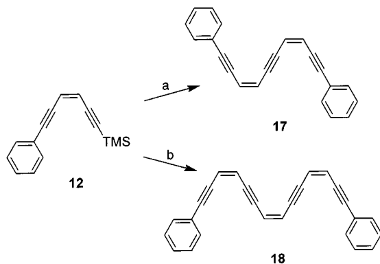
Scheme 4. Synthesis of 17 and 18 : a) \text{K}_2\text{CO}_3 , \text{CH}_3\text{OH}/\text{H}_2\text{O} , room temp., 6 h, then 11 (1.2 equiv.), \text{Pd}(\text{PPh}_3)_4 , \text{CuI} , n\text{BuNH}_2 , \text{C}_6\text{H}_6 , room temp., 24 h, 29% (2 steps); b) \text{K}_2\text{CO}_3 , \text{CH}_3\text{OH}/\text{H}_2\text{O} , room temp., 6 h, then 10 (0.4 equiv.), \text{Pd}(\text{PPh}_3)_4 , \text{CuI} , n\text{BuNH}_2 , \text{C}_6\text{H}_6 , room temp., 72 h, 6% (2 steps)
