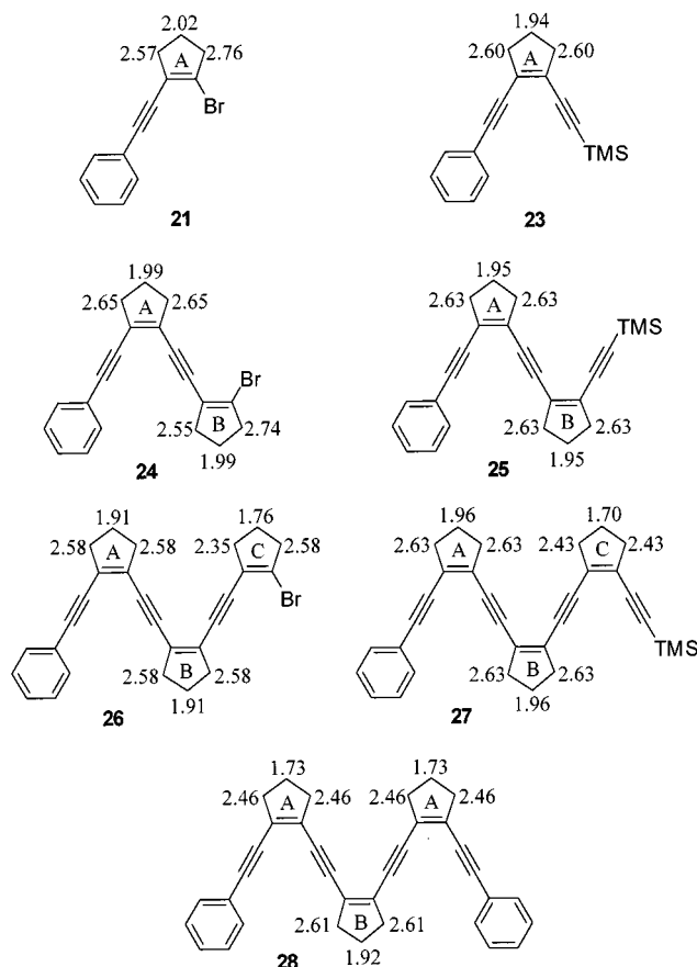
Figure 3. The ^1\text{H} NMR shifts of the cyclopentene rings of compounds 21 , 23 , 24 , 25 , 26 , 27 , and 28 ; upfield shifts of the cyclopentene C ring signals of 26 and 27 and of the A ring signals of the symmetrical compound 28 are apparent
