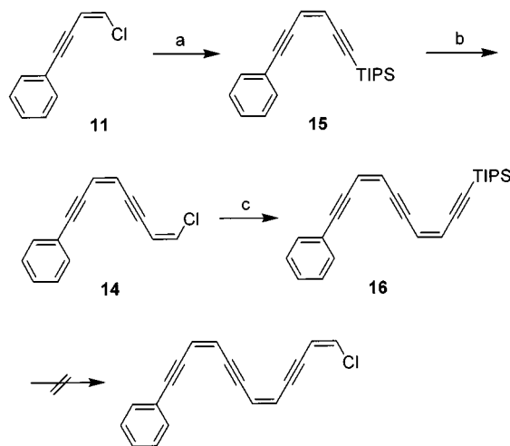
Scheme 3. Preparation of 16 : a) TIPS-acetylene (1.2 equiv.), Pd(PPh 3 ) 4 , CuI, n BuNH 2 , C 6 H 6 , room temp., 72 h, 94%; b) TBAF, THF/H 2 O, 3 h, then 10 (1.4 equiv.), Pd(PPh 3 ) 4 , CuI, n BuNH 2 , C 6 H 6 , room temp., 100 h, 41% (2 steps); c) TIPS-acetylene (1.5 equiv.), Pd(PPh 3 ) 4 , CuI, n BuNH 2 , C 6 H 6 , room temp., 20 h, 41%
