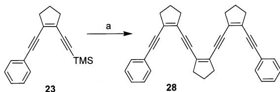
Scheme 8. Preparation of 28 : a) \text{K}_2\text{CO}_3 , \text{CH}_3\text{OH}/\text{H}_2\text{O} , room temp., 20 h, then 20 (0.45 equiv.), \text{PdCl}_2(\text{PPh}_3)_2 , \text{CuI} , n\text{BuNH}_2 , \text{C}_6\text{H}_6 , room temp., 20 h, 9% (2 steps)
