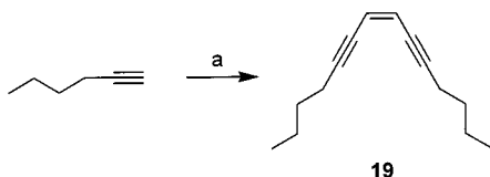
Scheme 5. Synthesis of 19 : a) 10 (0.5 equiv.), \text{Pd}(\text{PPh}_3)_4 , \text{CuI} , n\text{BuNH}_2 , \text{C}_6\text{H}_6 , room temp., 80 h, 80%
