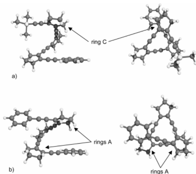
Figure 5. POV-ray representations of the PM3-optimized structures of 27 (a) and 28 (b) in the helical conformation (grey = carbon, white small = hydrogen, white large = silicon; left: side view of the helix; right: view through the helix; the spatial proximity to the phenyl rings of the cyclopentene A ring in 28 and the C ring in 27 is apparent)
