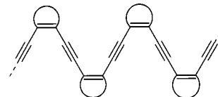
Figure 1. Stabilisation of the enyne backbones in cis -polydiacetylenes by introduction of ene moieties into a ring system
