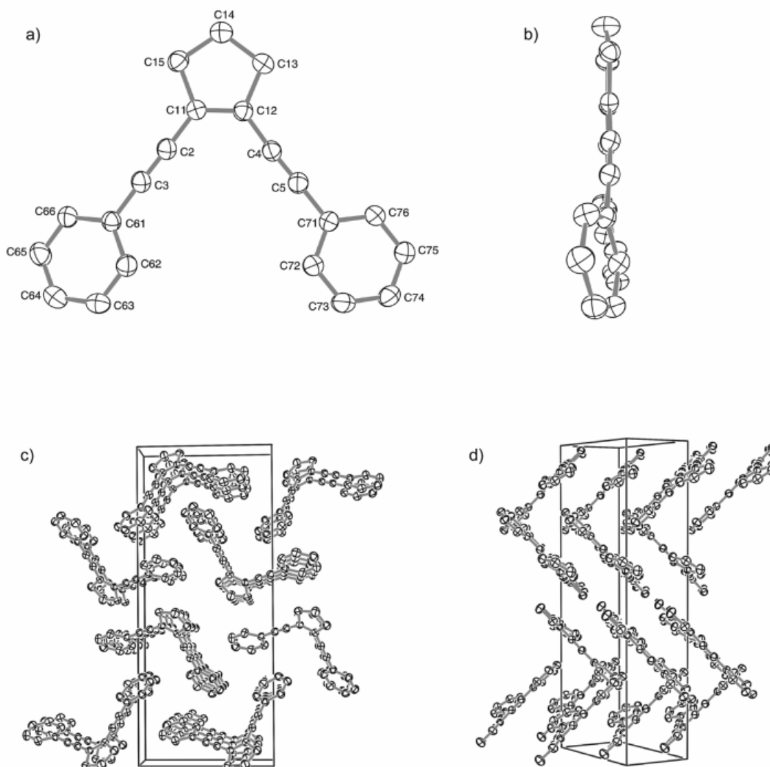
Figure 6. X-ray crystal structure of compound 22 (hydrogen atoms omitted for clarity): a) view of the molecule plane; b) side view; c) and d) arrangement of the molecules within the unit cell; selected bond lengths [Å] and angles [°]: C(3)–C(61) 1.432(3), C(2)–C(3) 1.199(3), C(2)–C(11) 1.420(3), C(11)–C(12) 1.346(3), C(11)–C(15) 1.503(3), C(14)–C(15) 1.510(3); C(2)–C(3)–C(61) 176.6(2), C(3)–C(2)–C(11) 178.0(2), C(12)–C(11)–C(2) 125.4(2), C(2)–C(11)–C(15) 123.3(2), C(12)–C(11)–C(15) 111.3(2), C(11)–C(15)–C(14) 104.5(2), C(13)–C(14)–C(15) 108.0(2)
