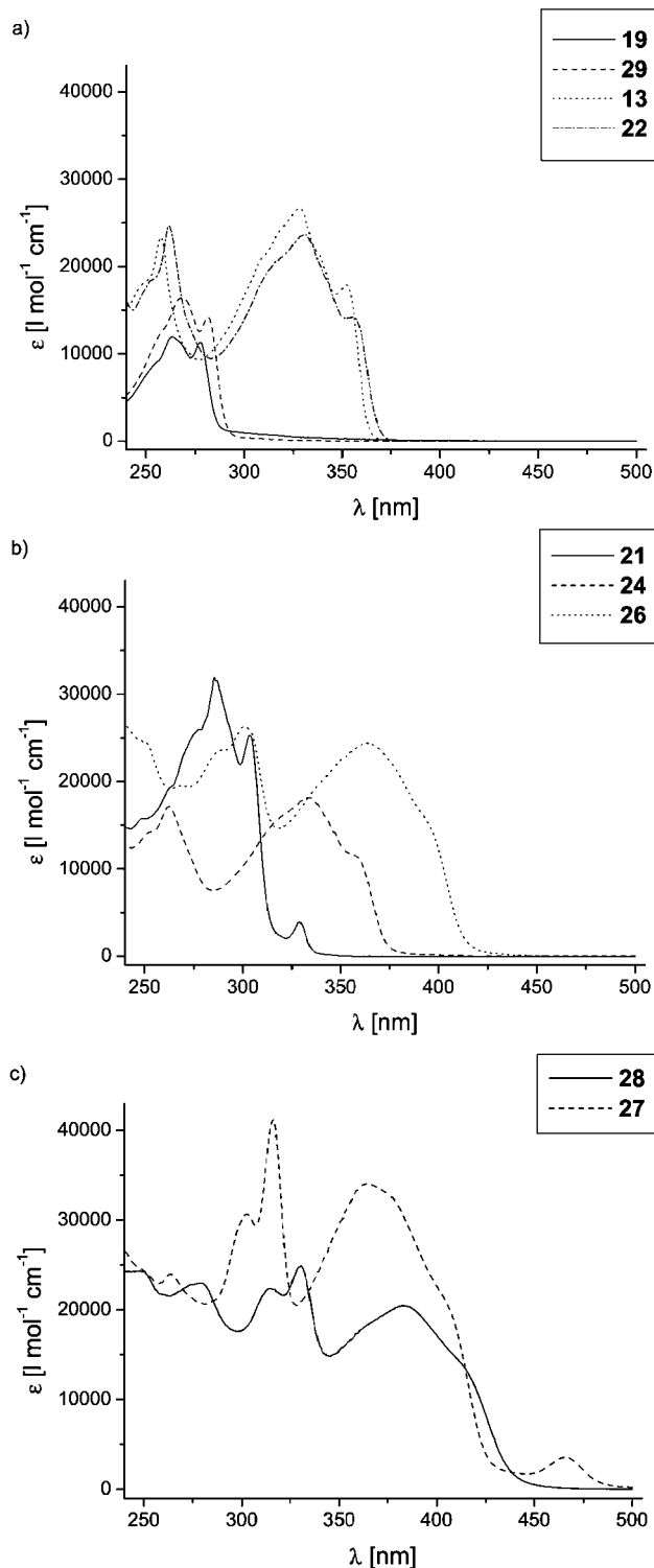
Figure 2. The UV spectra of selected compounds (further details in the text)
