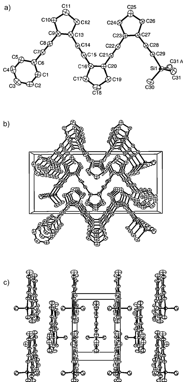
Figure 7. X-ray crystal structure of compound 27 (hydrogen atoms and solvent molecules omitted for clarity): a) view of the molecule plane; b) and c) arrangement of the molecules within the unit cell; selected bond lengths [Å] and angles [°]: C(20)–C(21) 1.410(5), C(21)–C(22) 1.211(5), C(22)–C(23) 1.398(5), C(23)–C(27) 1.361(5), C(27)–C(28) 1.414(5), C(28)–C(29) 1.195(5), Si(1)–C(29) 1.858(4), Si(1)–C(30) 1.850(5), C(23)–C(24) 1.535(6), C(24)–C(25) 1.518(8), C(25)–C(26) 1.528(7), C(26)–C(27) 1.518(6); C(21)–C(22)–C(23) 176.7(4), C(27)–C(23)–C(22) 126.7(3), C(23)–C(27)–C(28) 125.3(4), C(29)–C(28)–C(27) 179.7(4), C(27)–C(23)–C(24) 111.1(3), C(23)–C(27)–C(26) 110.7(3), C(25)–C(24)–C(23) 105.1(4), C(24)–C(25)–C(26) 107.2(5), C(27)–C(26)–C(25) 105.8(4), C(28)–C(29)–Si(1) 173.9(4), C(30)–Si(1)–C(29) 106.8(2)
